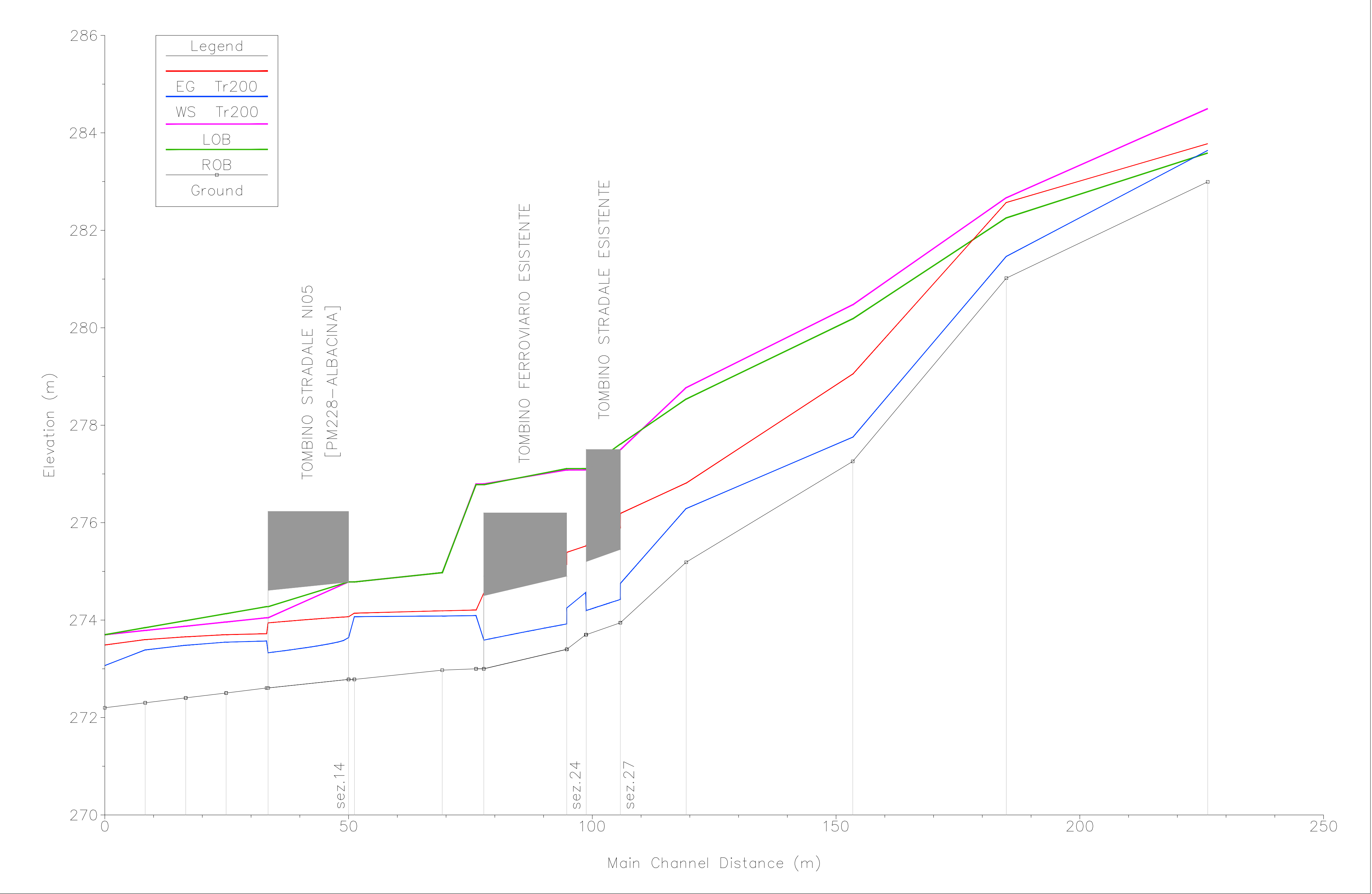
TOMBINO IN01: PROFILO RIGURGITO POST OPERAM - Scala 1:500/1:50
