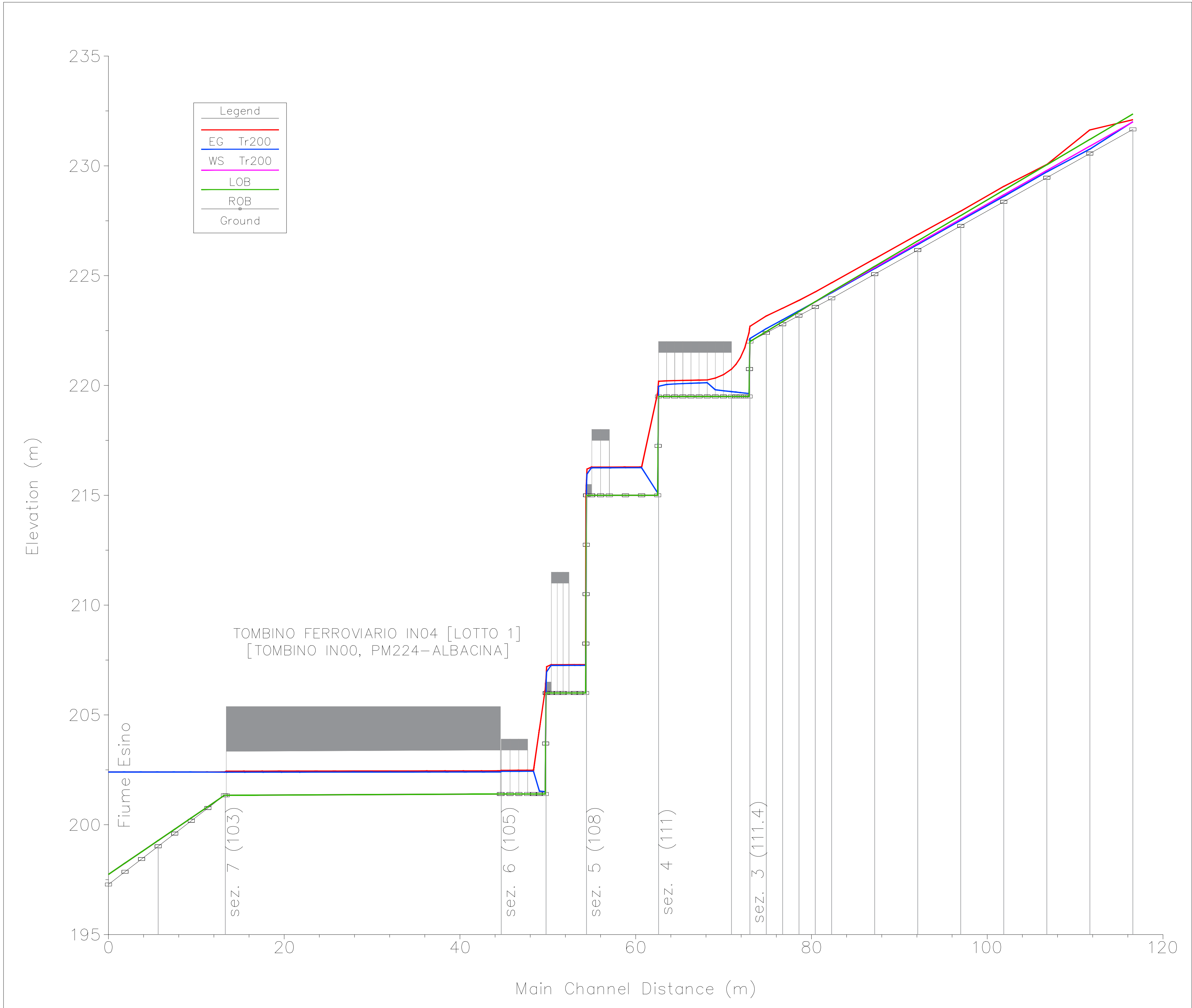
TOMBINO IN04: PROFILO RIGURGITO POST OPERAM - Scala 1:250/1:100
